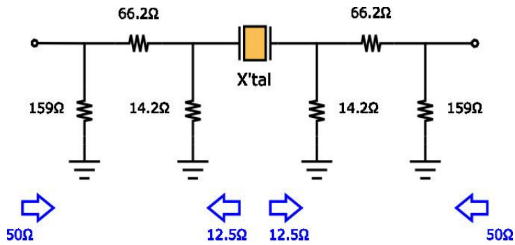
Pi Network test fixture [IEC 444]
